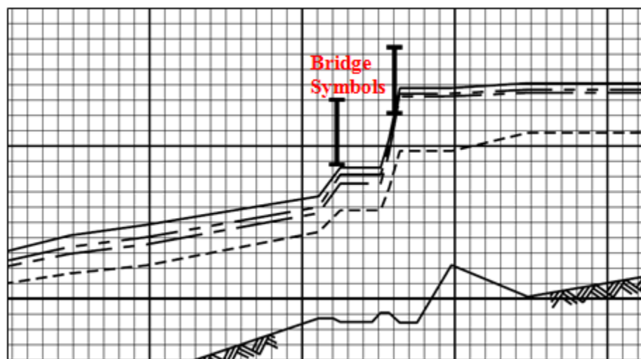
Figure 6: Bridge Symbol Example on Profile
